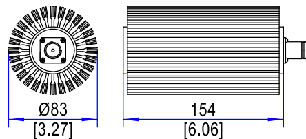
Outline B N-Type Female Connector
