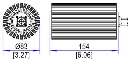
Outline A N-Type Male Connector
