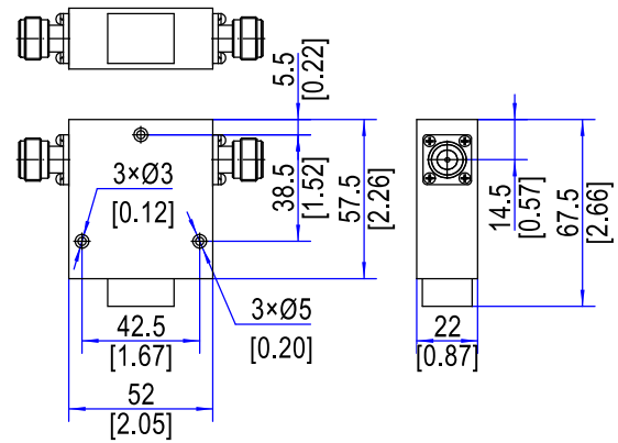
Outline B
