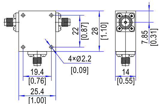
Outline B: SMA Connector
