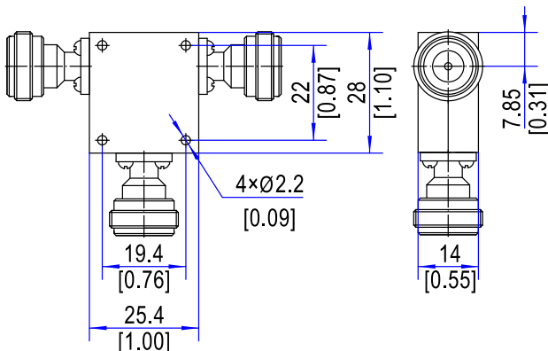
Outline A: N-Type Connector
