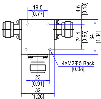
Outline A: N-Type Connector
