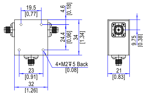
Outline B: SMA Connector
