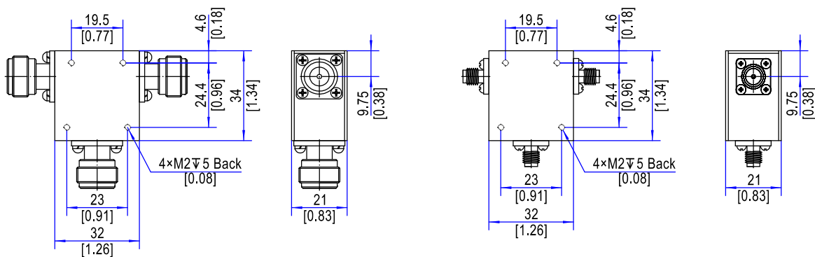
Outline A: N-Type Connector
