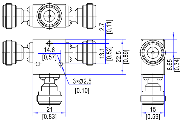
Outline A: N-Type Connector
