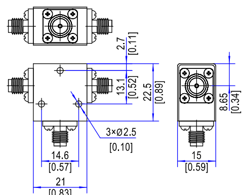
Outline B: SMA Connector
