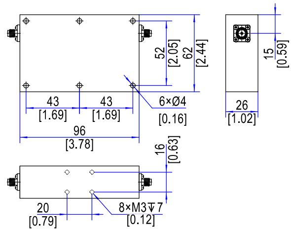
Outline B SMA Connector
