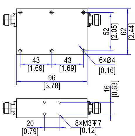
Outline A N-Type Connector
